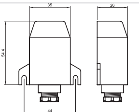
Dimensions, ETF-5xx
