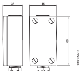
Dimensions, ETF-11xx
